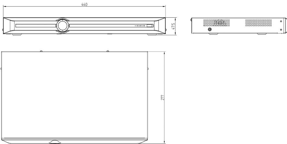
NVR202P Outline Dimensions
