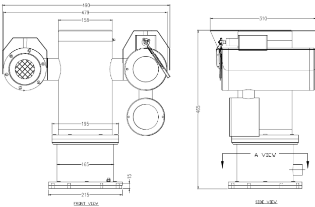
SX1PTZD-LEDW-G Outline Dimensions
