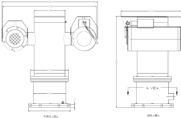
SX1PTZD-W-G Outline Dimensions
