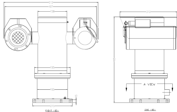
SX1PTZD-W-GL Outline Dimensions
