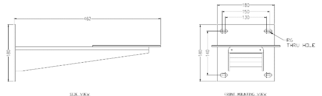
WB-SX1PTZ - Wall Bracket Outline Dimensions
