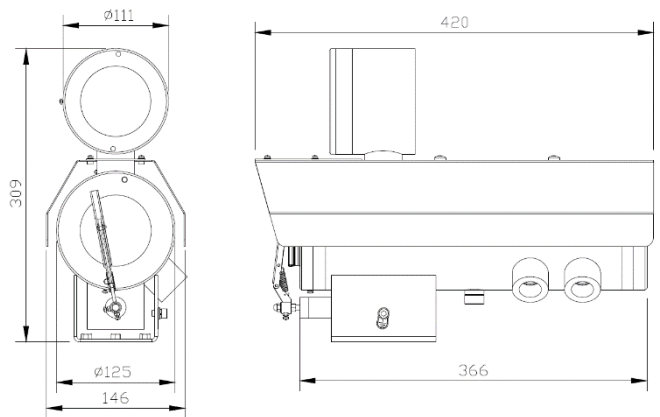
SS1CH-LEDW Outline Dimensions
