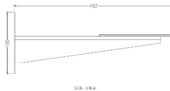
WB-SS1PTZ - Wall Bracket Outline Dimensions
