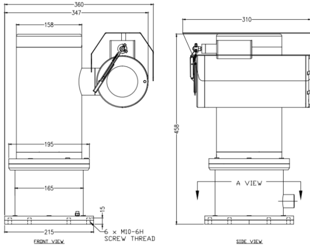
SS1PTZ-W Outline Dimensions
